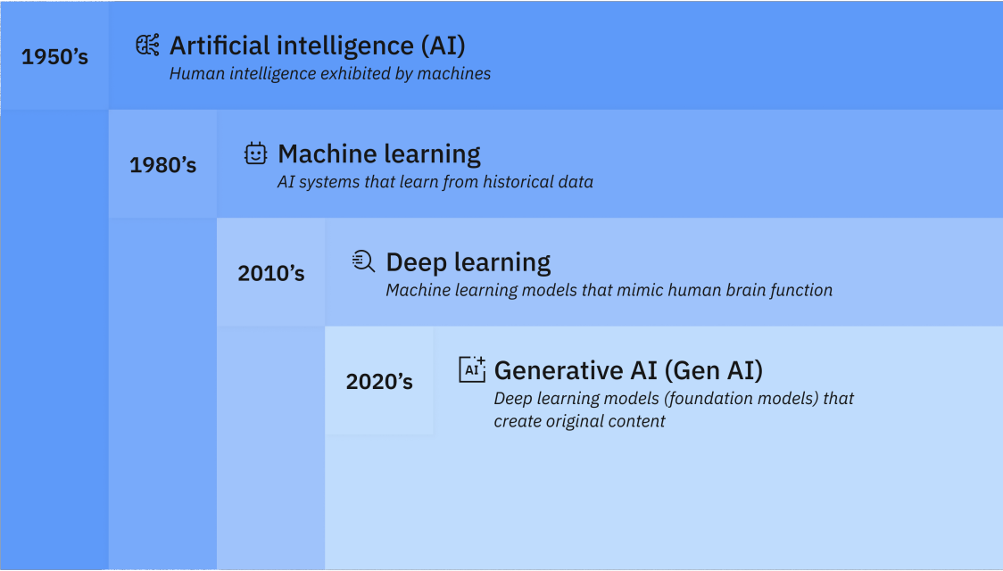
Figure 1.1: diagram-comparing-ai-ml-deep-learning-genai
